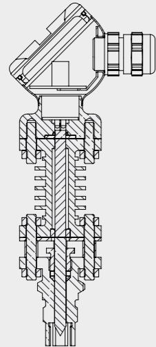
Mounting thread with cooling element
